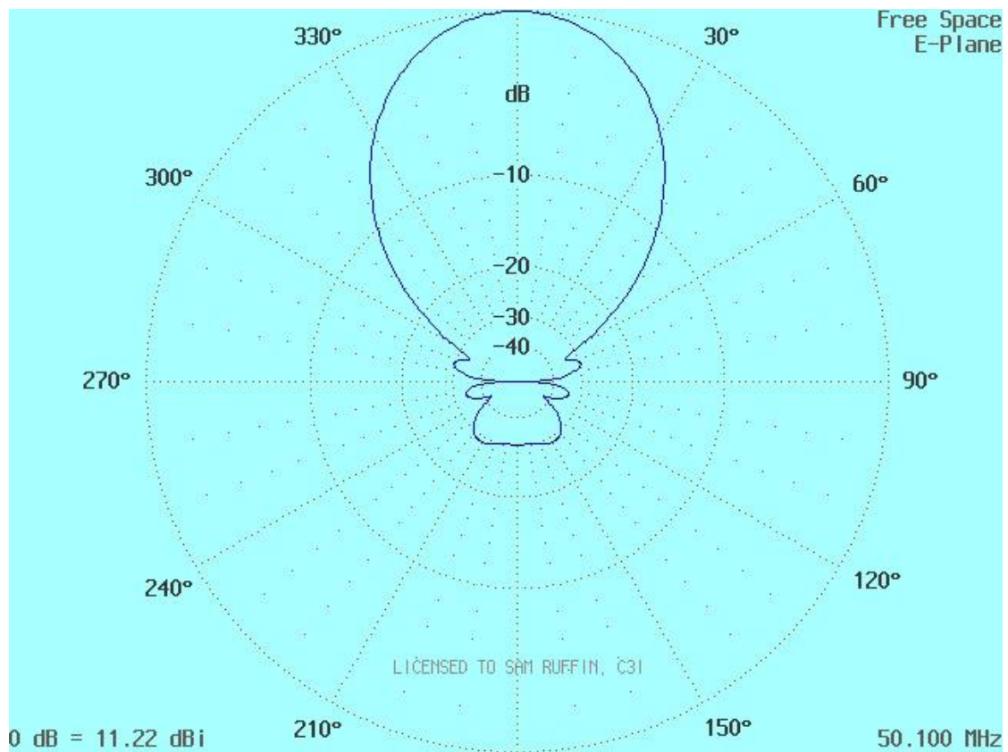
DSEJX6-50 E-Plane Computer – Generated Polar Plot
